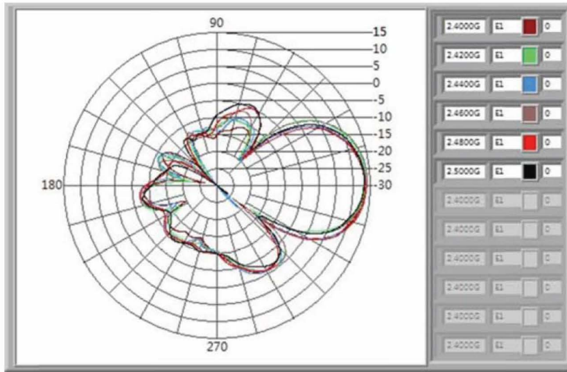
Vertical Pattern E-plane
